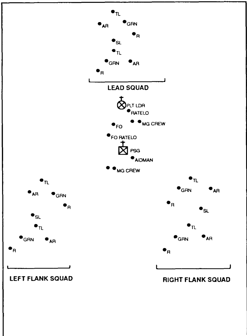
Figure 2-15. Platoon wedge.
